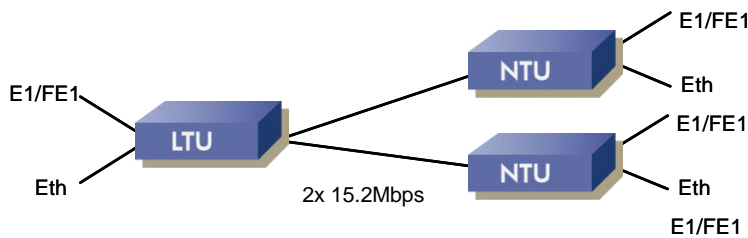
Point-to-Multipoint Application
